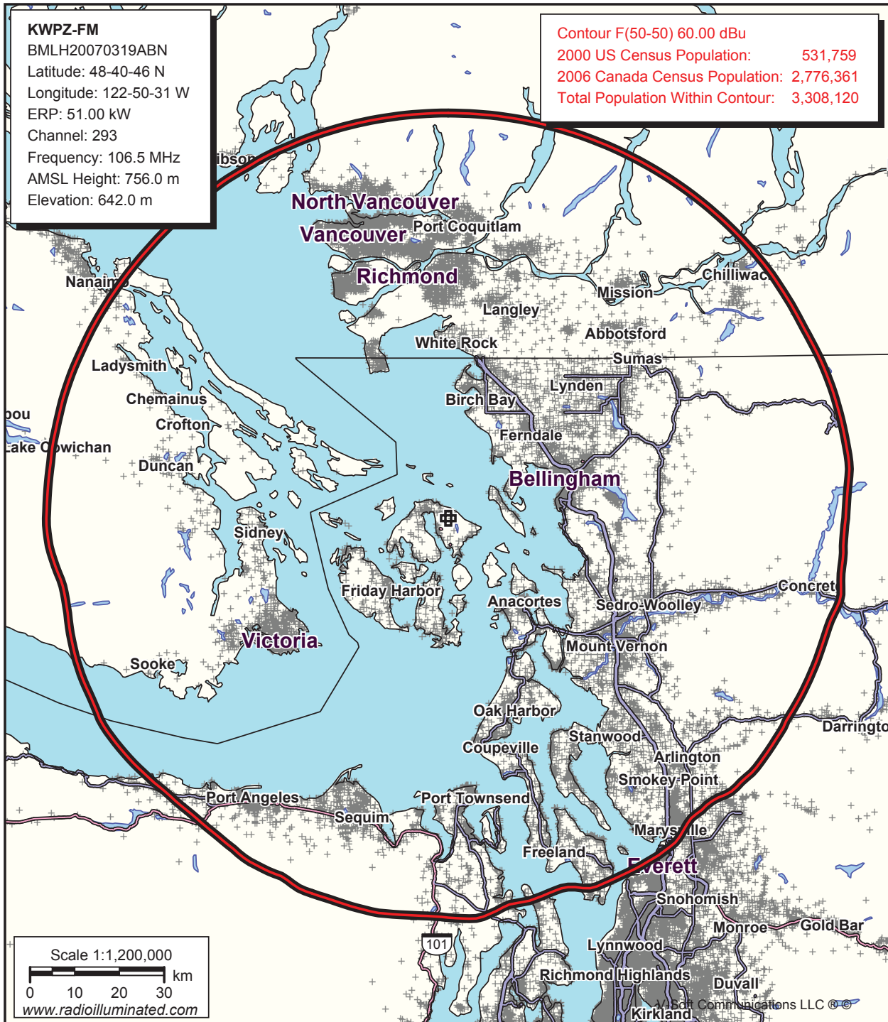
Census Scattergram
